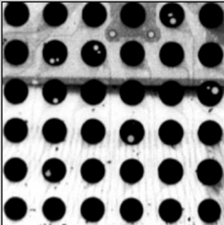
BGA Voiding
